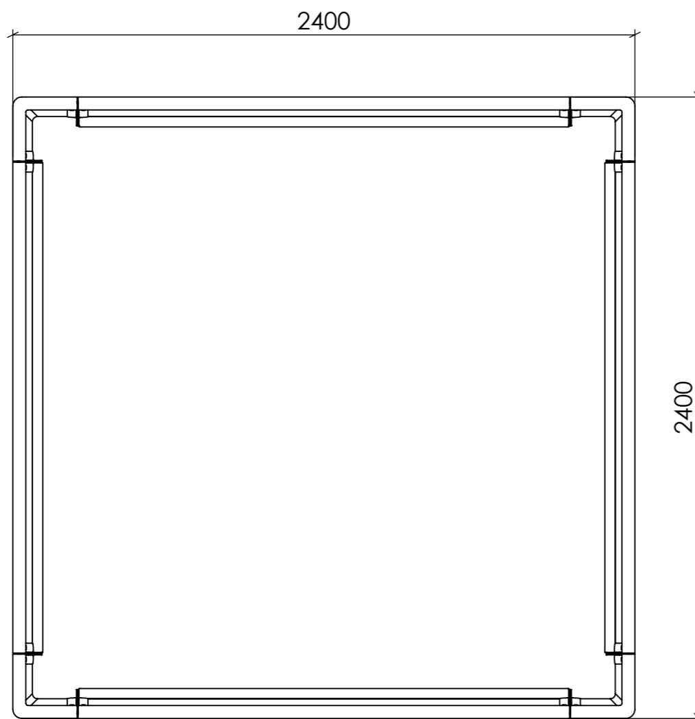
TOPPVY
