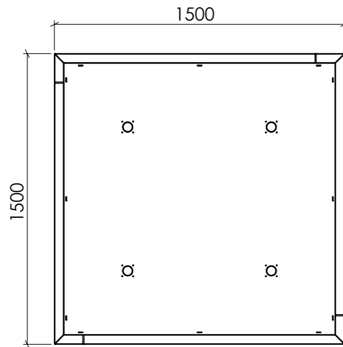
TOPPVY
